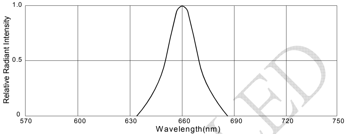
Fig.1 Relative Radiant Intensity VS. Wavelength
