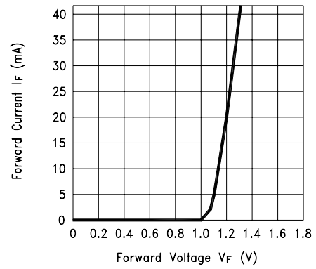
Fig.2 Forward Current I F vs. Forward Voltage V F
