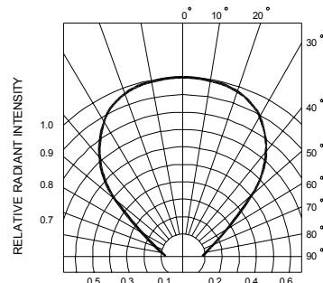
RADIATION DIAGRAM
